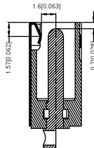
SECTION B-B
